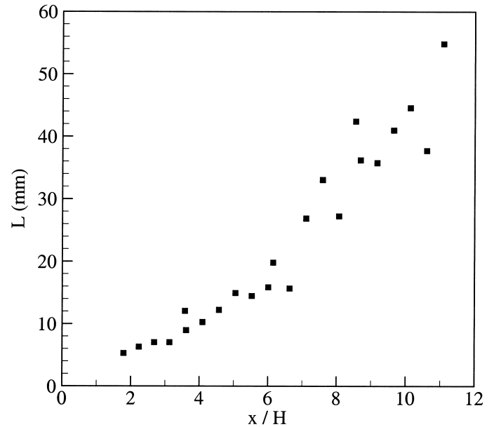
Fig. 5. Variation of spanwise integral length scale with distance from the source.
